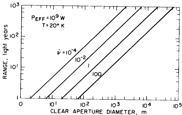
Figure 6-5. Doppler limited ranges.
