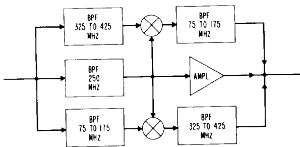
Figure 10-9. Channel interchanger.
